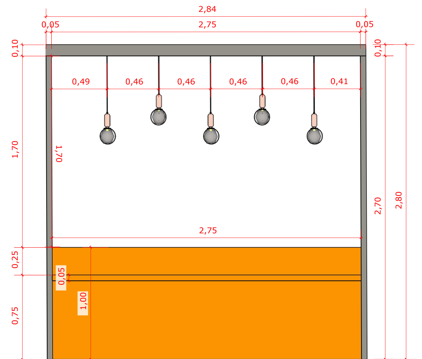
VISTA FRONTAL
